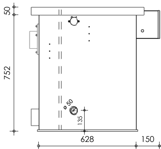
Right-side view
